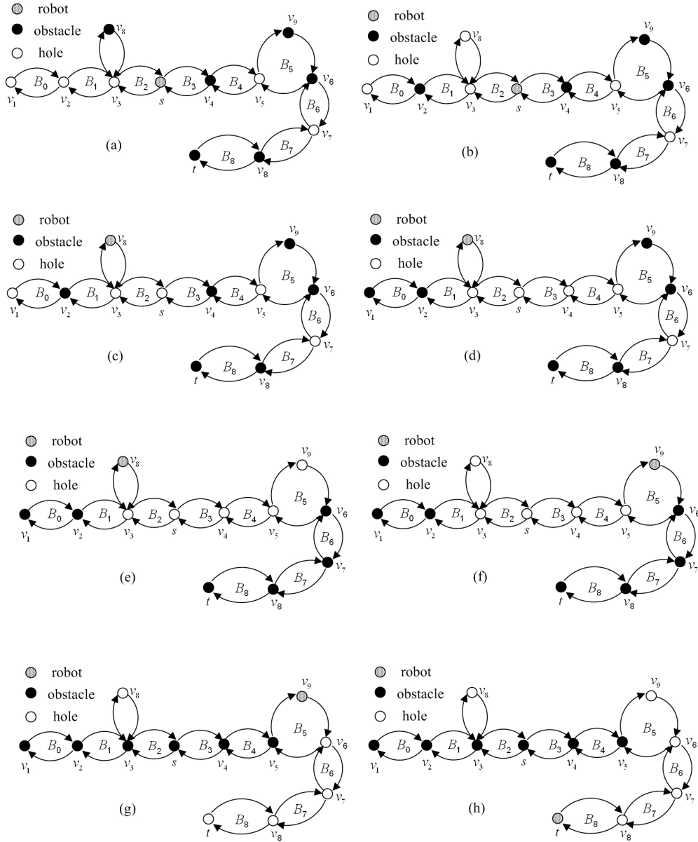
Figure 9. Example: motion planning on a strongly connected digraph: Case II
