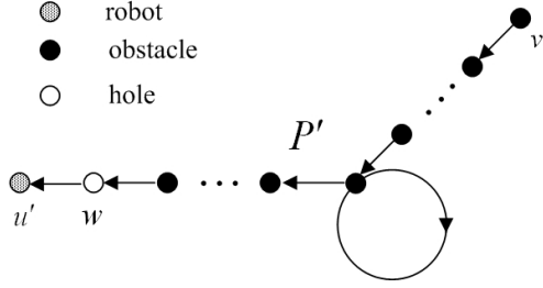
Figure 6. The case that the hole and t are in P_{j_0} different from u' and v' , s \in D_{j_0-1} , and s \neq u'
