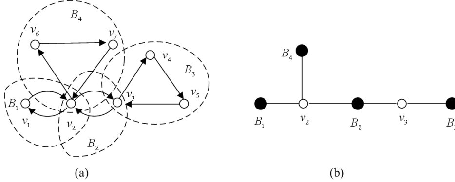
Figure 4. Example: strongly-biconnected-component graph
