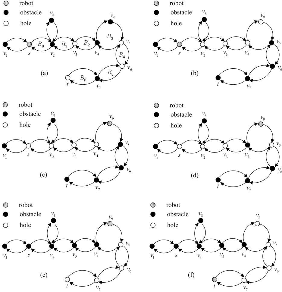
Figure 8. Example: motion planning on a strongly connected digraph: Case I
