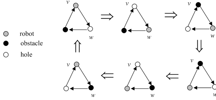
Figure 5. Restoration by rotating the objects in a cycle
