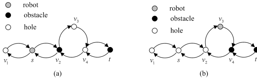
Figure 7. Example: t -side of the robot
