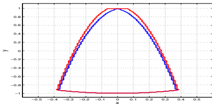
Fig. 3. An illustration of comparison of the computed lower robust controlled invariant set \mathcal{R}^- and upper robust controlled invariant set \mathcal{R}^+ for Example 1. Red and blue curves denote the boundaries of computed sets \mathcal{R}^- and \mathcal{R}^+ , respectively.
