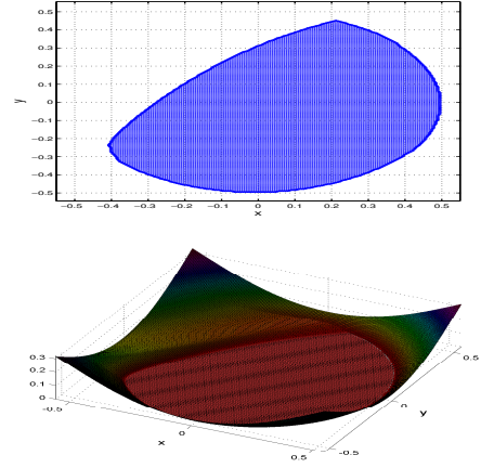
Fig. 4. Above: The blue region denotes the computed lower robust controlled invariant set \mathcal{R}^- and upper robust controlled invariant set \mathcal{R}^+ . Below: An illustration of level sets of the computed upper value function V^-(\mathbf{x}) and upper value function V^+(\mathbf{x}) for Example 2.
