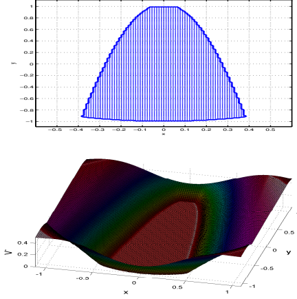
Fig. 1. Above: The blue region denotes the computed lower robust controlled invariant set \mathcal{R}^- for Example 1. Below: An illustration of level sets of the computed lower value function V^-(\mathbf{x}) .
