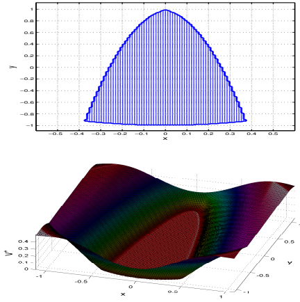
Fig. 2. Above: The blue region denotes the computed upper robust controlled invariant set \mathcal{R}^+ for Example 1. Below: An illustration of level sets of the computed upper value function V^+(\mathbf{x}) .
