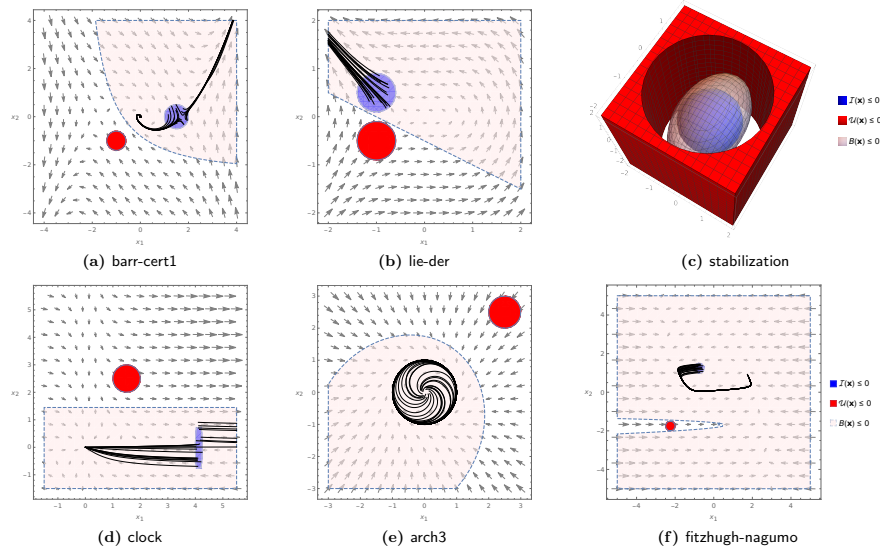
Fig. 3: Phase portraits of another selected set of examples with the synthesized invariant barrier certificates. The arrows indicate the vector field (hidden in 3D-graphics for a clear presentation) and the solid curves are randomly sampled trajectories.
