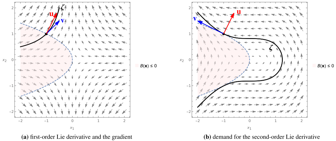
Fig. 6. An illustration of how Lie derivatives capture the tendency of trajectories in terms of a polynomial function B(\mathbf{x}) . \zeta : the system trajectory passing through (-1, 1) ; \mathbf{v} : the evolution direction per the vector field at (-1, 1) ; \mathbf{u} : the gradient of B(\mathbf{x}) at (-1, 1) .
