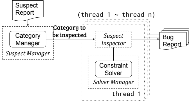
Figure 4: Structure of the parallel inspector
