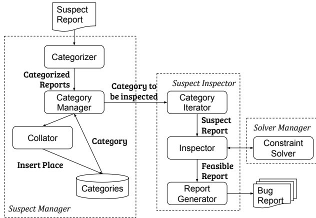
Figure 3: Structure of the categorized inspector
