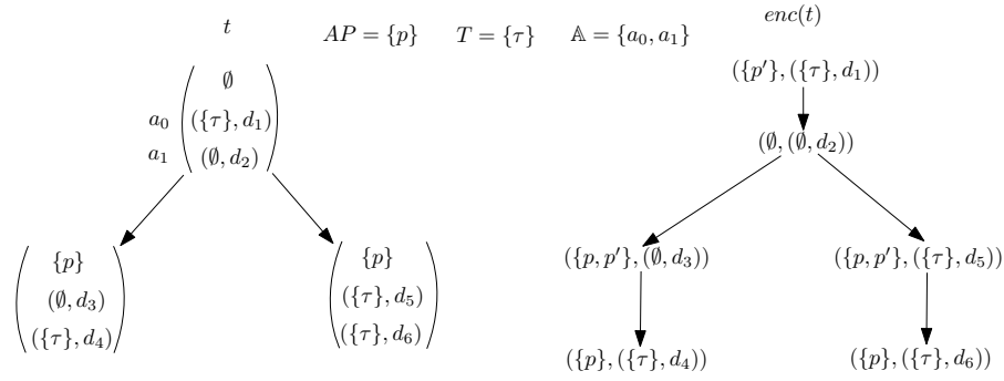
Figure 3: \mathbb{A}' -attributed encoding of \mathbb{A} -attributed data trees
