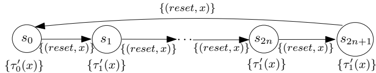
Figure 2: The Kripke Structure.
