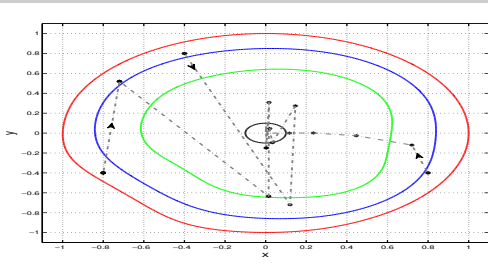
Fig. 3. An illustration of the computed p -reach-avoid sets for Example 2. The black curve denotes the boundary of the target set \mathcal{T} . The red, blue and green curves denote the boundaries of the computed inner-approximations of the 0.0-, 0.25-, and 0.6-reach-avoid sets respectively. The gray-black curves denote the trajectories starting from (-0.8, -0.4)^\top , (-0.4, 0.8)^\top and (0.8, -0.4)^\top with \theta(l) \equiv 0 respectively.
