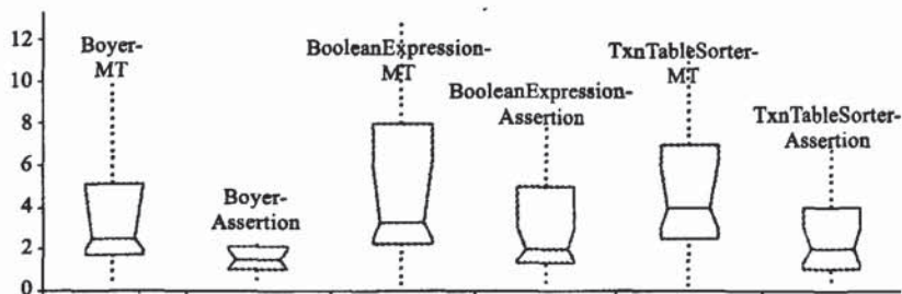
Fig.2 Box-and-Whisker plots of time costs for applying mt and assertion checking
