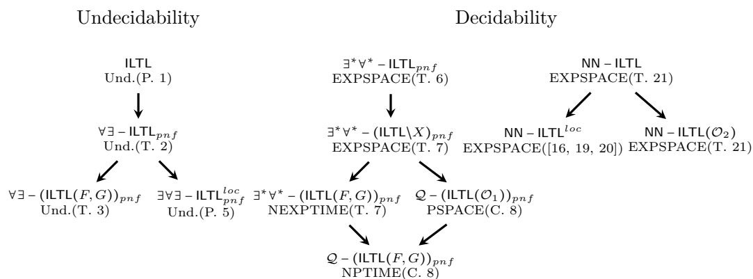
■ Figure 1 Summary of the results: Und. (Undecidable), T. (Theorem), C. (Corollary), \mathcal{Q} \in \{\exists\forall^*\} \cup \{\exists^*\forall^k \mid k \in \mathbb{N}\} , \mathcal{O}_1 is \{X, F, G\} or \{U, R\} , \mathcal{O}_2 is \{X, F, G\} or \{U, R\} or \{F, G\} .
