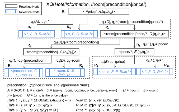
Fig. 4. Example of XPath Rewriting Graph.
