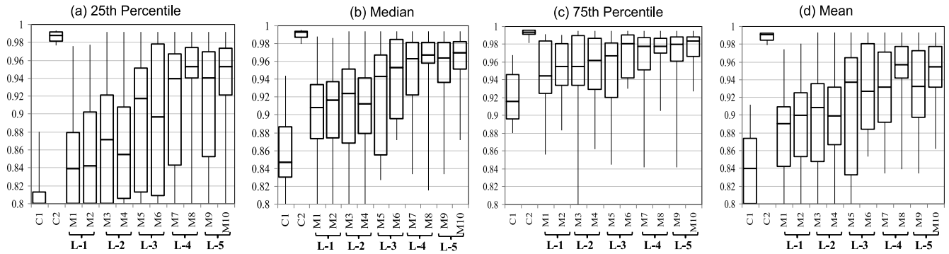
Fig. 8. Overall comparisons in terms of APFD measure.
