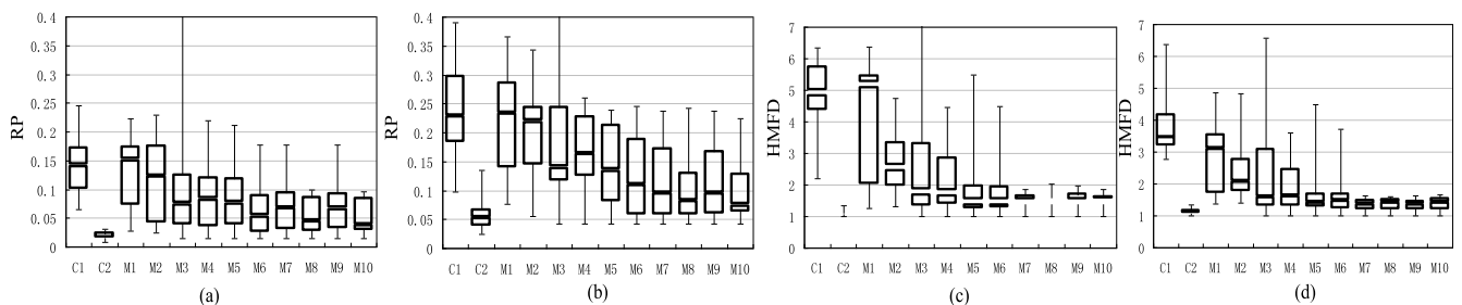
Fig. 10. Results of techniques in terms of (a) RP using tool-generated test suites, (b) RP using manual test suites, (c) HMFd using tool-generated test suites, and (d) HMFd using manual test suites.
