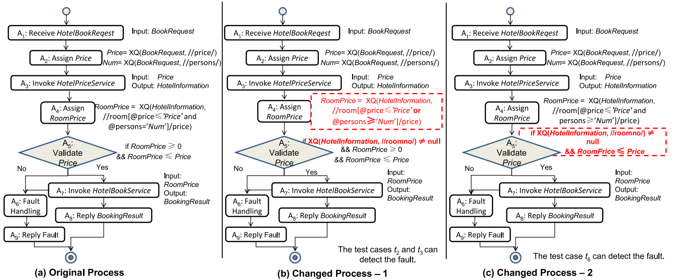
Fig. 5. Activity diagrams of business process HotelBooking .
