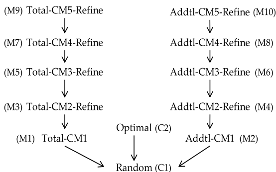
Fig. 7. Subsumption hierarchy of test case prioritization techniques.
