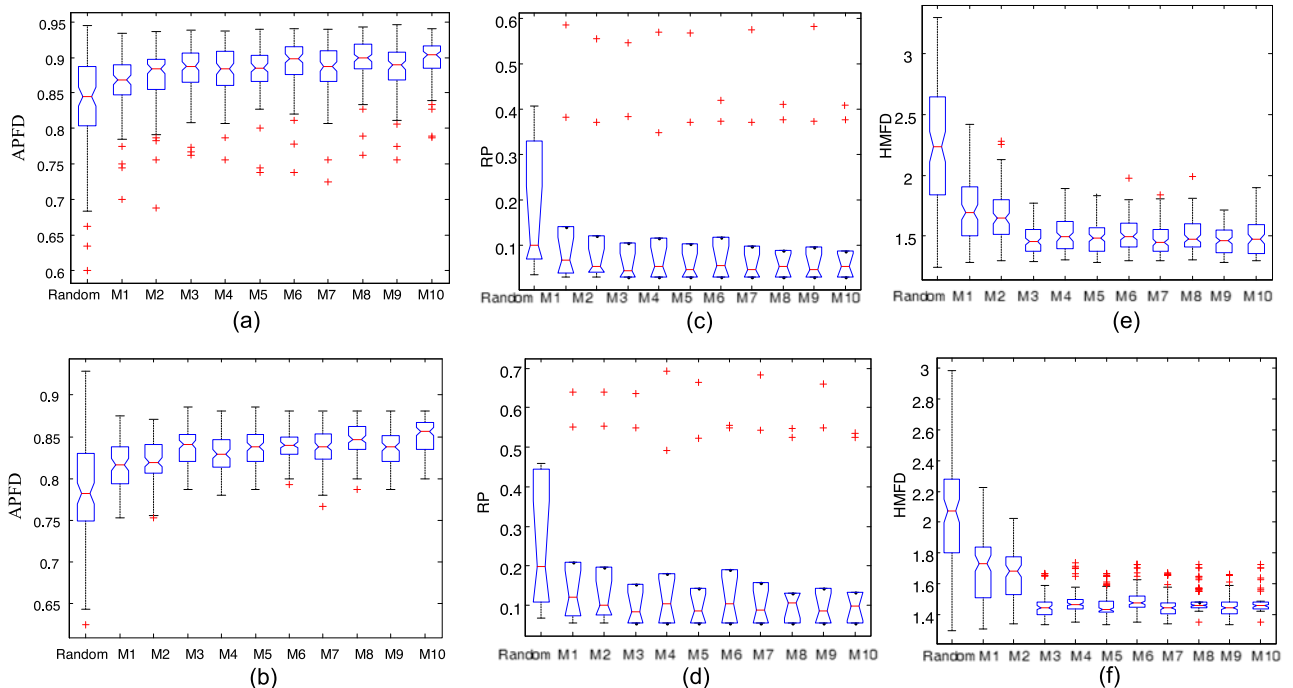
Fig. 11. Comparisons in case study, in terms of (a) APFD using tool-generated test suites, (b) APFD using manual test suites, (c) RP using tool-generated test suites, (d) RP using manual test suites, (e) HMFd using tool-generated test suites, and (f) HMFd using manual test suites.
