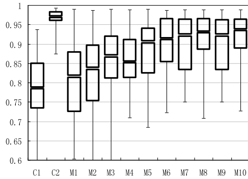
Fig. 9. Overall comparisons in terms of mean APFD using manual test suites.
