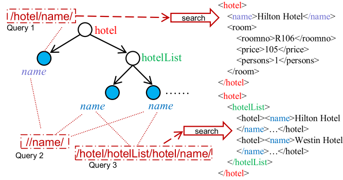
Fig. 2. Effects of the structure of an XML message on different XPath queries to locate hotels using hotel name.
