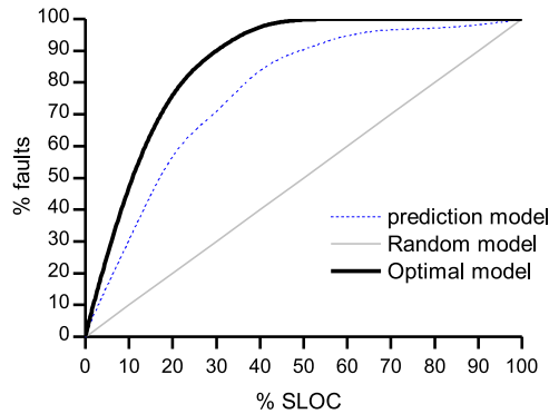
Fig. 1. SLOC-based Alberg diagram.
