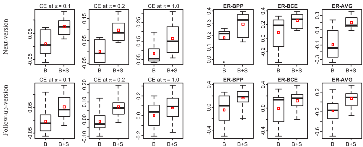
Fig. 6. Ranking/Classification performance comparison under cross-version prediction: the “B” model versus the “B+S” model on the continuous versions of the Bash system.
