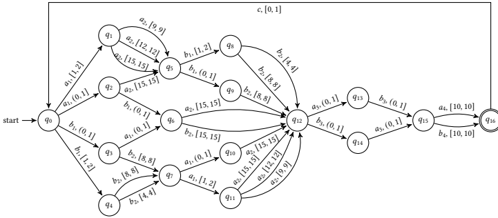
(d) The learnt NRTA \mathcal{H} excluding the "sink" location and relevant transitions
