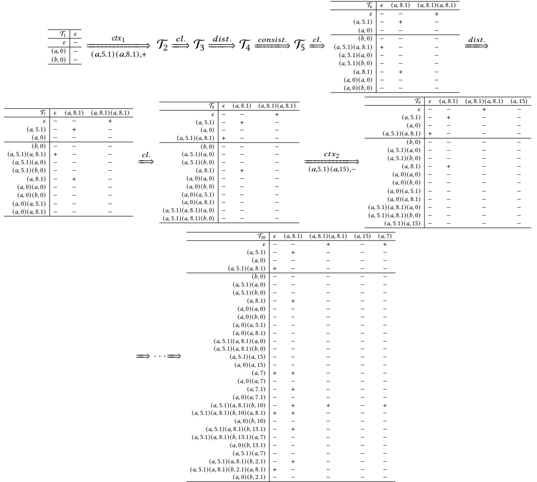
Fig. 6. Some of the table instances generated in the process of learning NRTA \mathcal{A} in Fig. 2.
